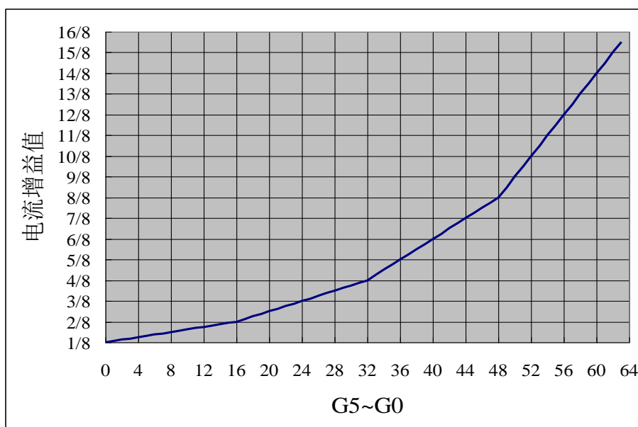
Fig. SM16380SC I OUT 电流增益调节曲线
